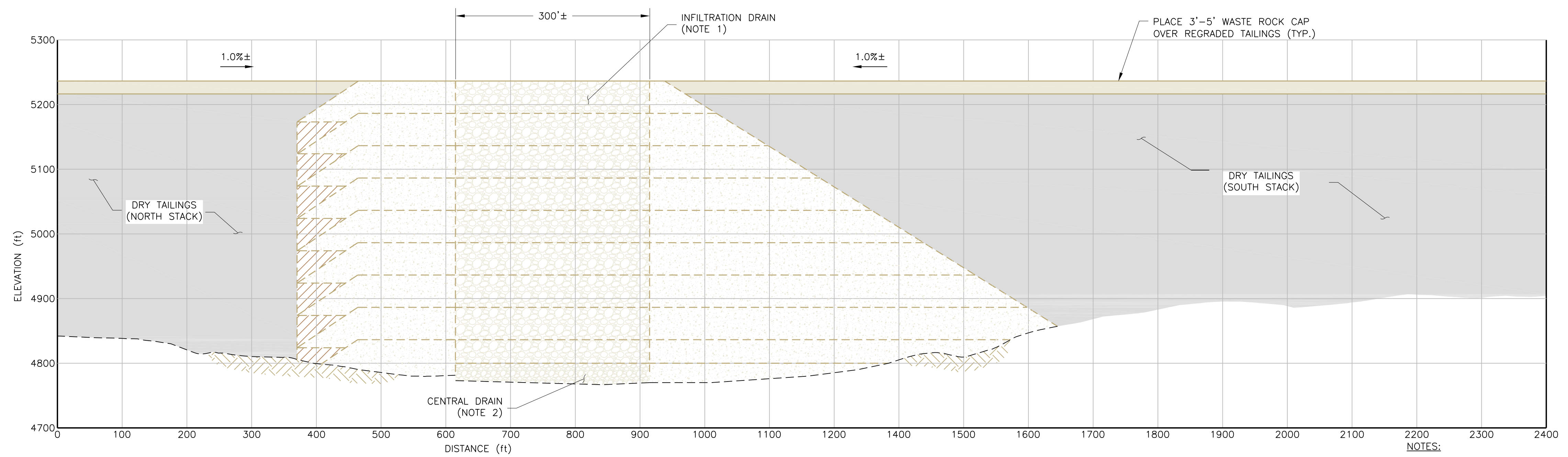
B 07/08 CENTRAL DRAIN CROSS SECTION
