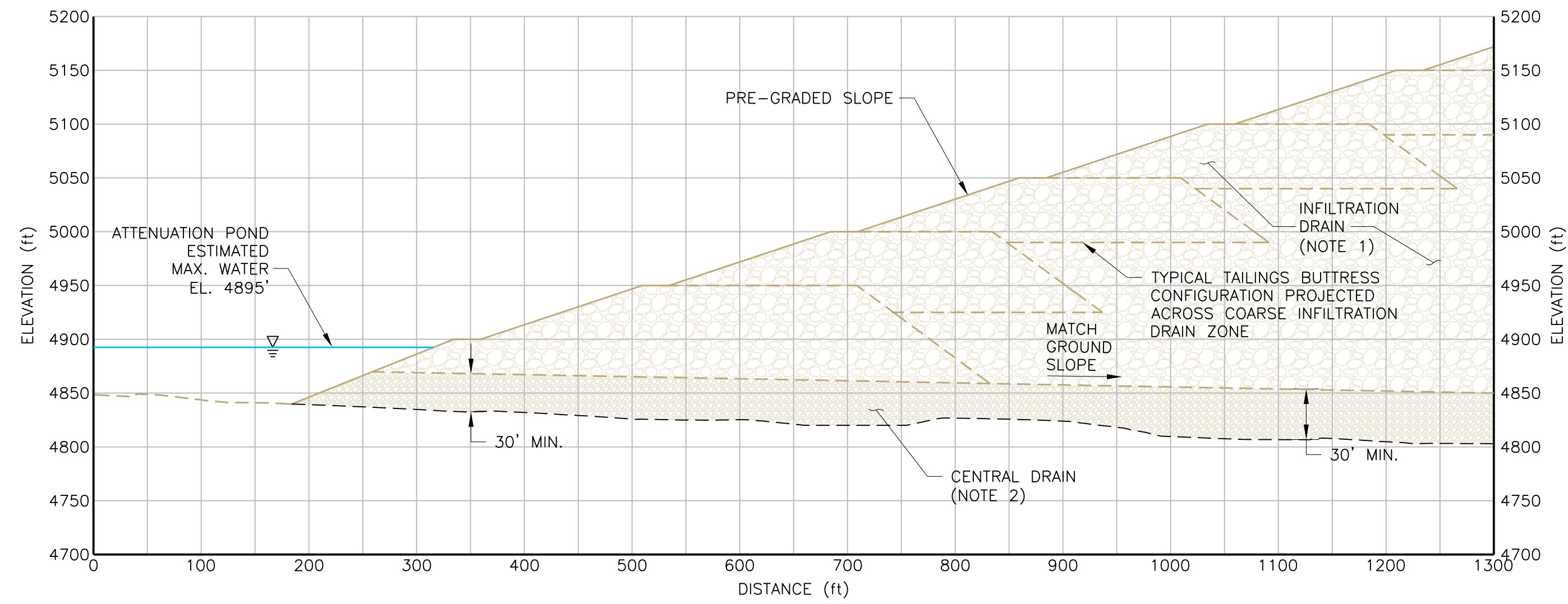
A 07/08 CENTRAL DRAIN CROSS SECTION
