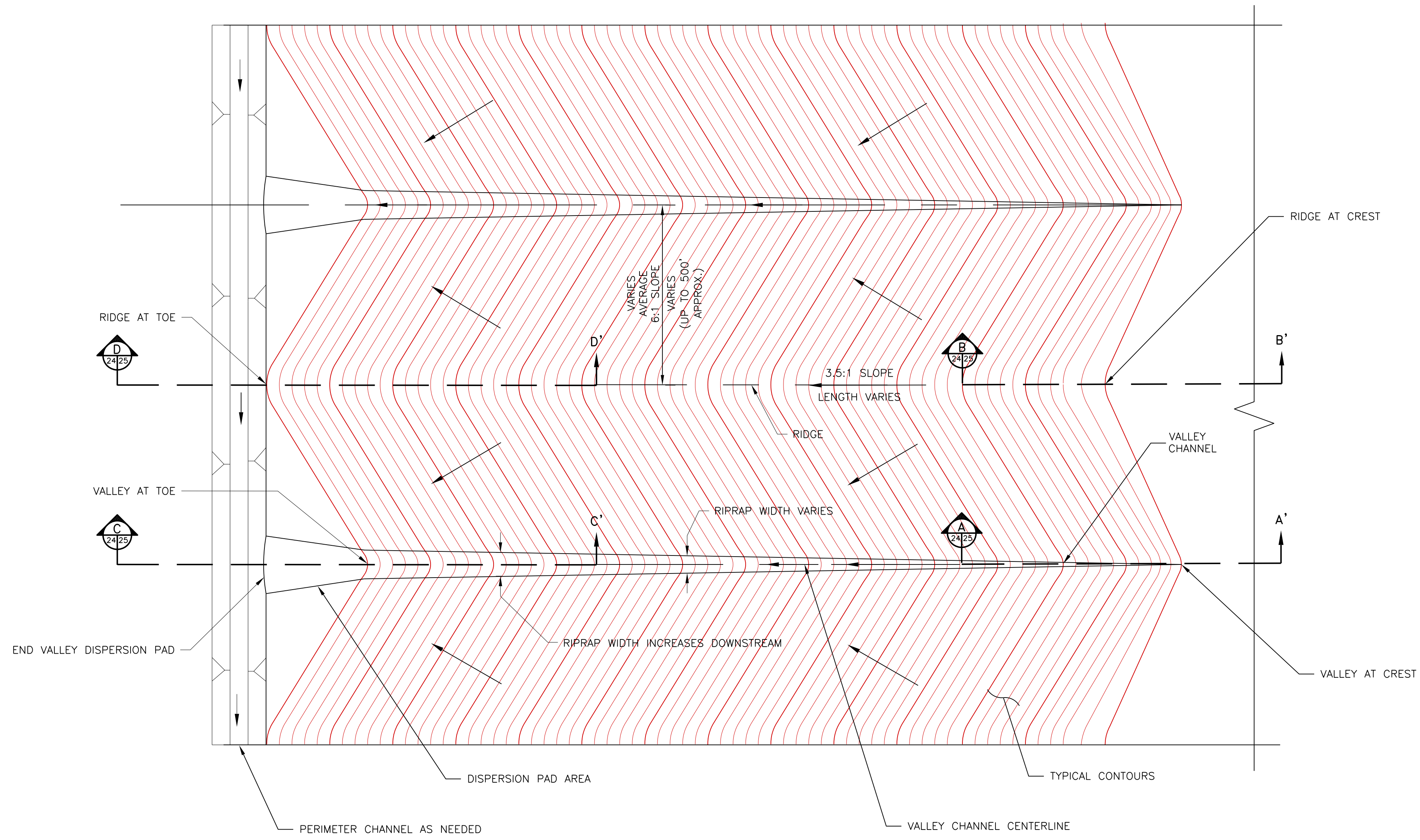
TYPICAL RIDGE AND VALLEY - PLAN VIEW
